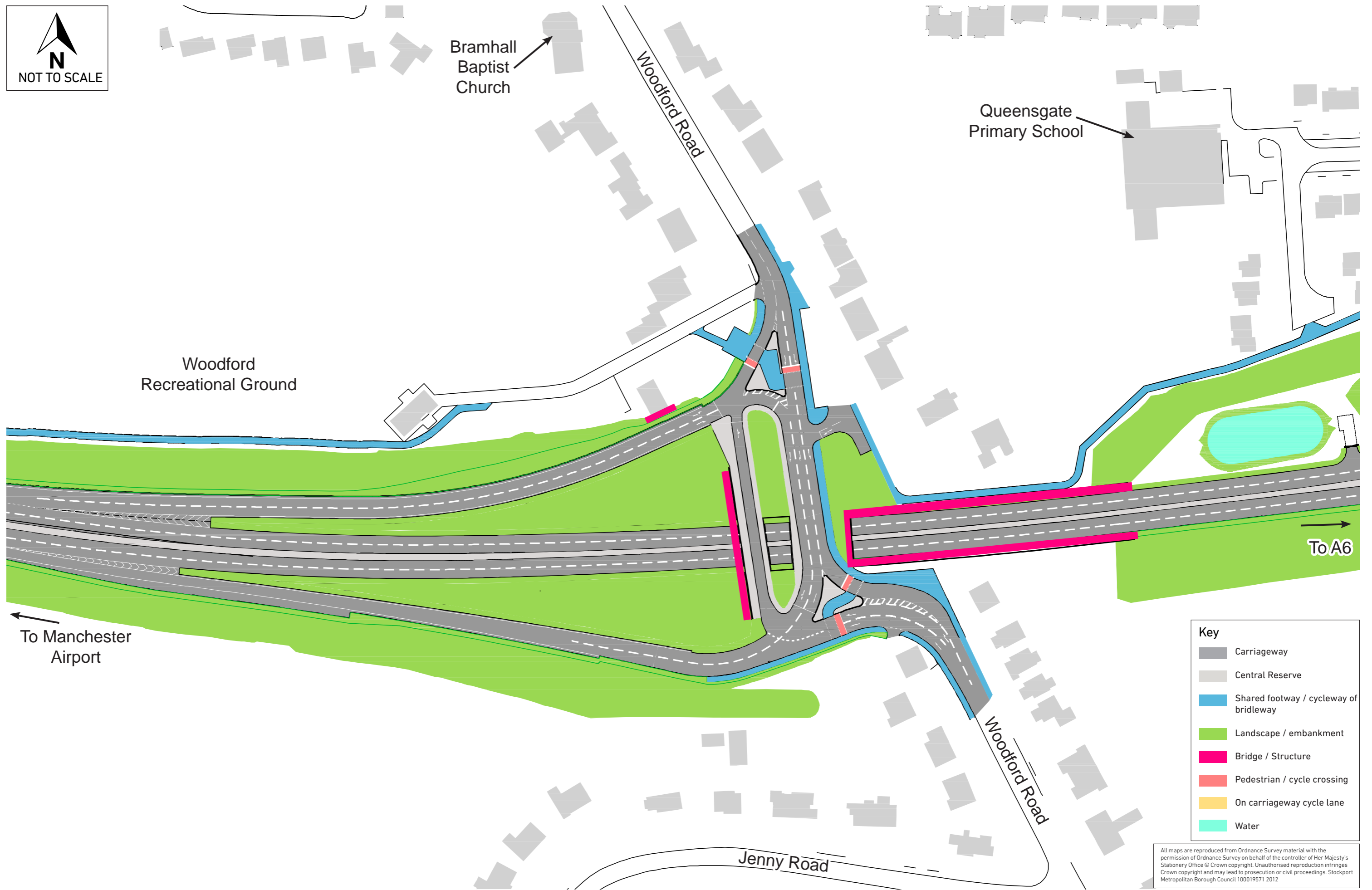
LOCATION 3: Woodford Road, Bramhall : Option 1: Scheme passes under a realigned Woodford Road with new traffic lights controlled junction introduced.
