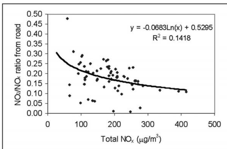
Figure C3 The Relationship Between the Ratio of NO x and NO 2 Contributions From Road Traffic and Total NO x Concentrations
